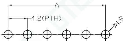
PCB LAYOUT
