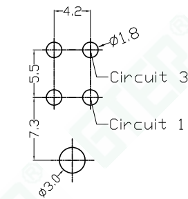
2x02P PCB LAYOUT
