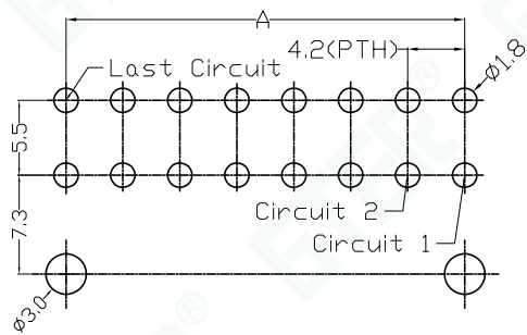
2x03P-2x12P PCB LAYOUT
