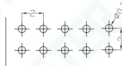
DIP SIDE ENTRY TYPE PCB LAYOUT
